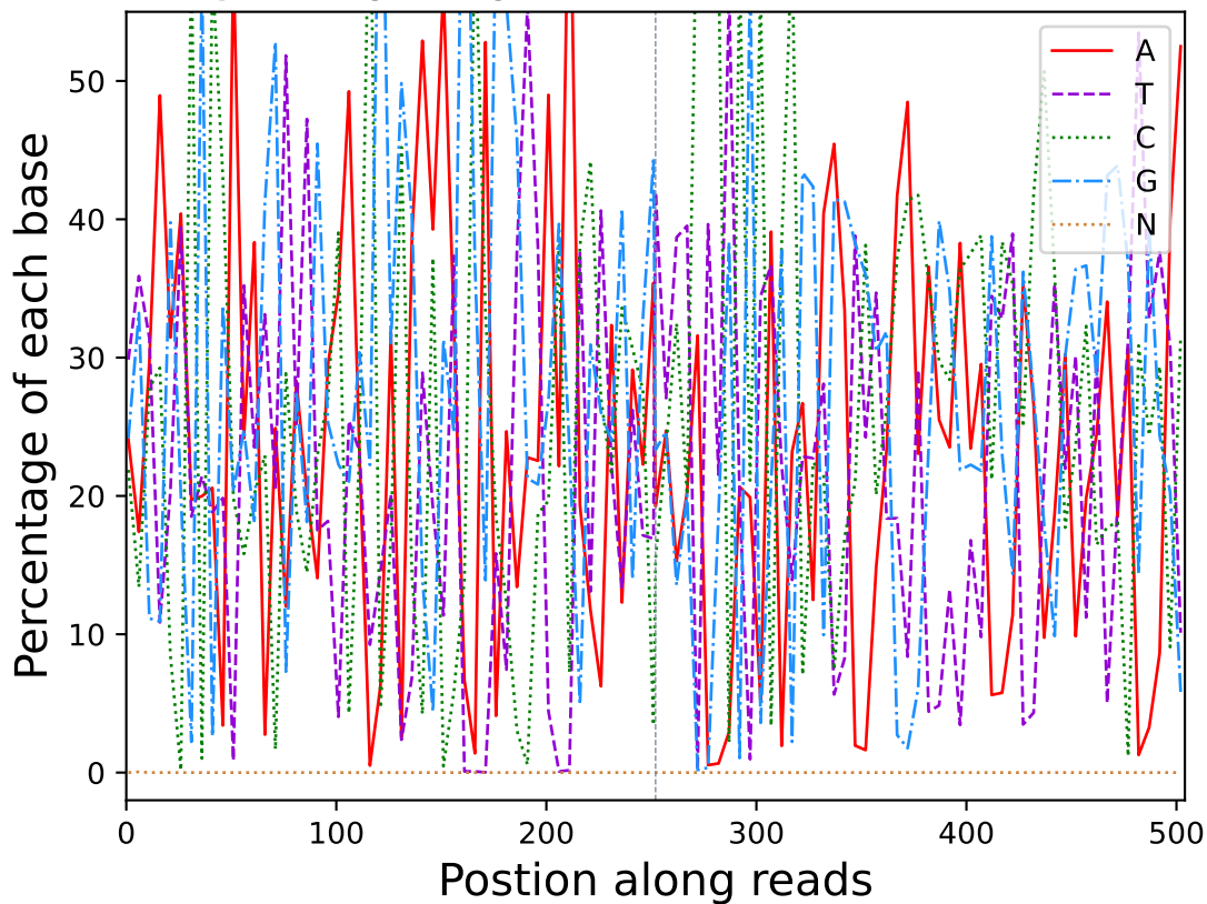
Base percentage along reads (CKH1)
